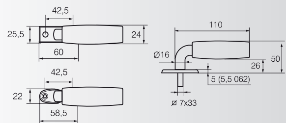
Brass/Larch handle
