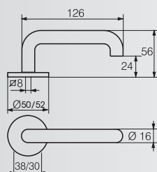
Handles available in brass or aluminium
