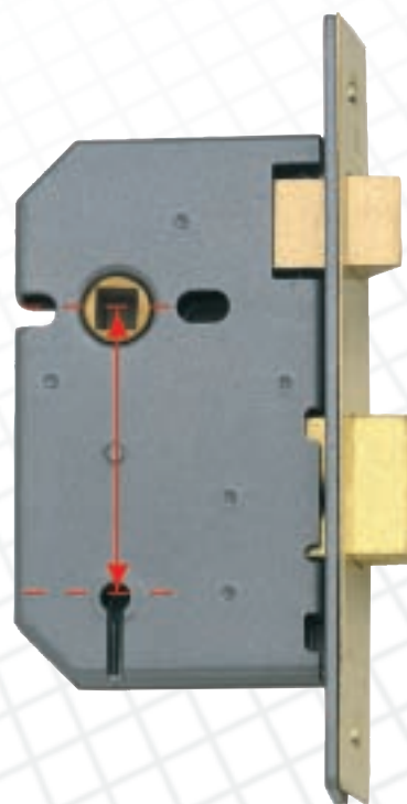
Centres (57mm)
