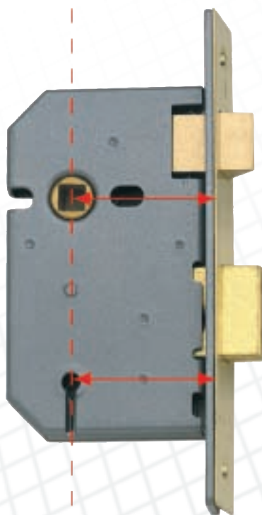
Backset (44.5mm).
