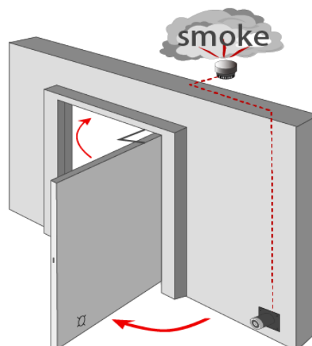
DH503 / DH503B Wall mounted W/Release switch (DH503B only)
