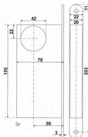
LOCKCASE DIMENSIONS (mm) 50mm backset (78mm case depth)
