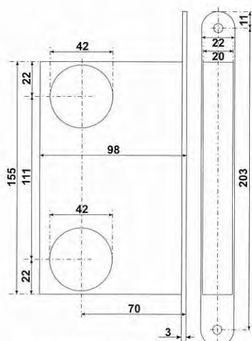
LOCKCASE DIMENSIONS 70mm backset (98mm case depth)
